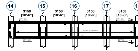
FLOOR BEAM ON G.L. F & B (2 NO)
