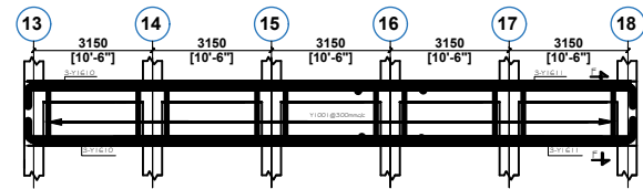
FLOOR BEAM ON G.L. L (1 NO)
