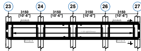
FLOOR BEAM ON G.L. F (1 NO)
