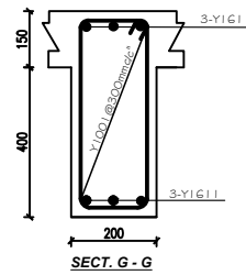
FLOOR BEAM ON G.L. A & O (2 NO)
