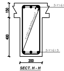
FLOOR BEAM ON G.L. A & H (2 NO)
