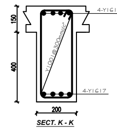
FLOOR BEAM ON G.L. 23, 25, 26 & 27 (4 NO)
