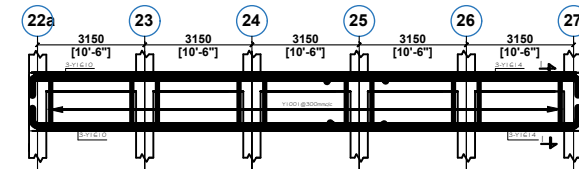
FLOOR BEAM ON G.L. A & N (2 NO)
