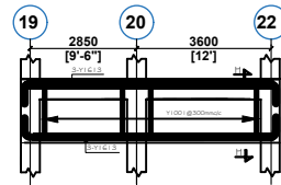
FLOOR BEAM ON G.L. A & H (2 NO)
