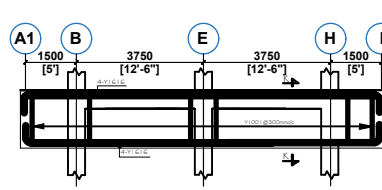
FLOOR BEAM ON G.L. 13, 14, 15, 16, 17, 18, 21, 22, 23 & 24 (10 NO)
