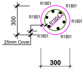
SECTION 8-8/9-9
