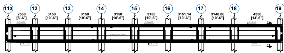
FLOOR BEAM ON G.L. B, E & H (3 NO)
