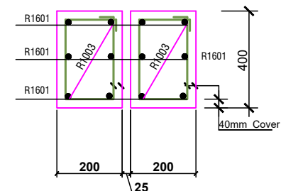
SECTION 5 - 5
