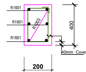
SECTION 4 - 4
