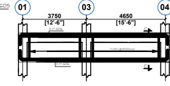
FLOOR BEAM ON G.L. A1 & C (2 NO)
