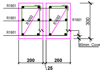
SECTION 3 - 3
