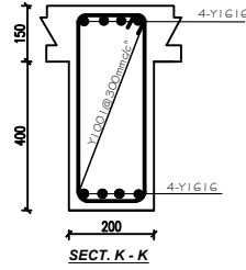
FLOOR BEAM ON G.L. 13, 14, 15, 16, 17, 18, 21, 22, 23 & 24 (10 NO)
