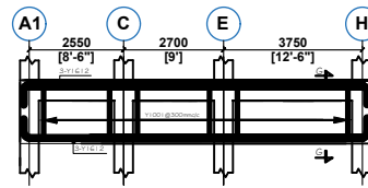
FLOOR BEAM ON G.L. 01, 03 & 04 (3 NO)
