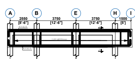
FLOOR BEAM ON G.L. 11a, 12, 19a, 20, 25 & 26 (6 NO)
