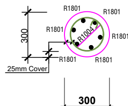
SECTION 2 - 2
