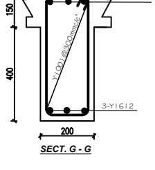
FLOOR BEAM ON G.L. 01, 03 & 04 (3 NO)
