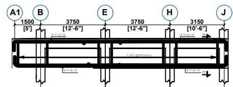
FLOOR BEAM ON G.L. 01, 07, 09, 10 & 11 (5 NO)
