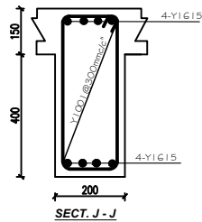
SECT. J - J
