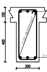
SECT. D - D
