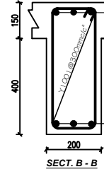
SECT. B - B
