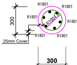
SECTION 8-8/9-9
