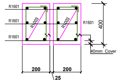
SECTION 5 - 5
