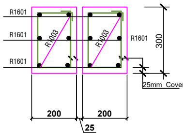
SECTION 10-10/11-11
