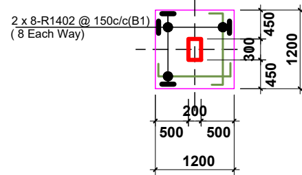
COL. BASE TYPE 'B1' ( 71 No. THUS )
