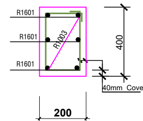
SECTION 16-16/17-17
