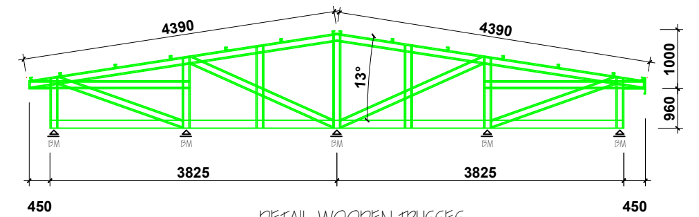
DETAIL WOODEN TRUSSES (TRUSS TYPE 'A')
