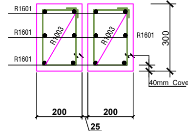
SECTION 3 - 3
