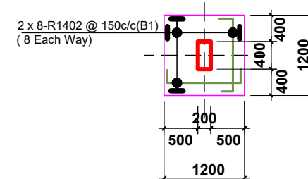
COL. BASE TYPE 'B4' ( 34 No. THUS )
