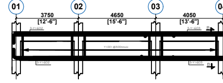
FLOOR BEAM ON G.L. D & G (2 NO)
