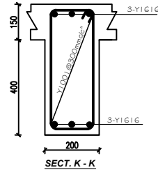
FLOOR BEAM ON G.L. 02, 03 & 04 (3 NO)
