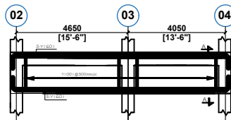
FLOOR BEAM ON G.L. N (1 NO)
