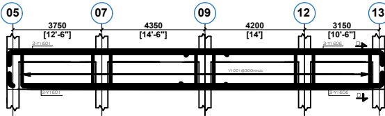
FLOOR BEAM ON G.L. D & G (2 NO)
