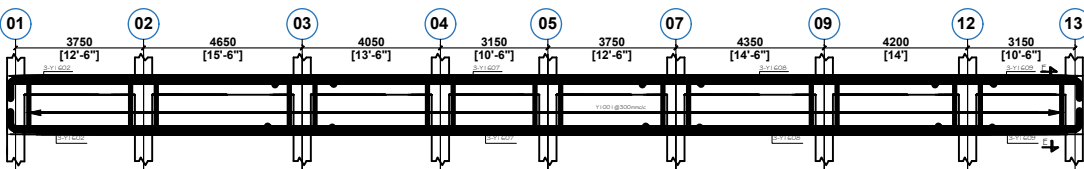
FLOOR BEAM ON G.L. A (1 NO)
