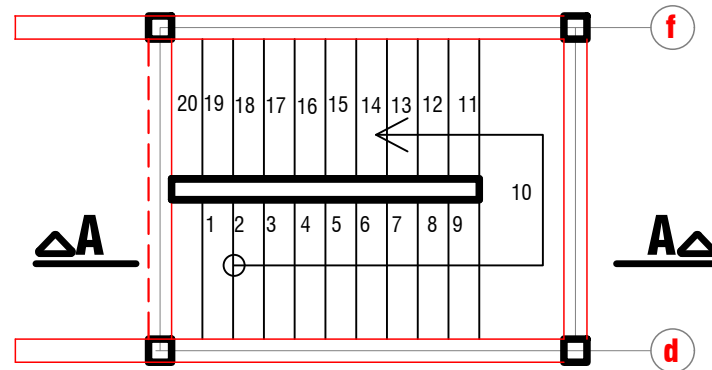
G.A. STAIRCASE FROM GROUND FLOOR TO ROOF FLOOR
