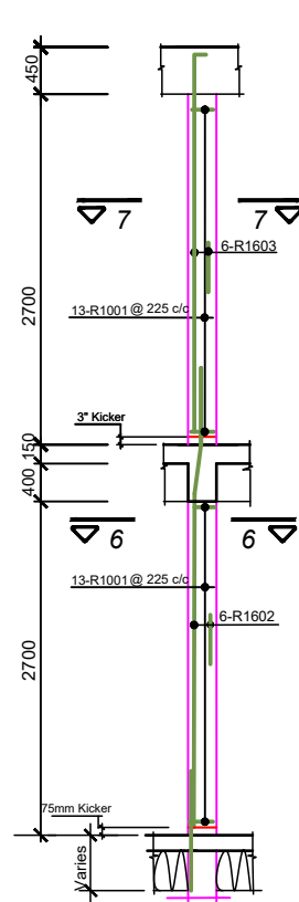
COLUMN TYPE 'C1' ( 54 No. THUS )
