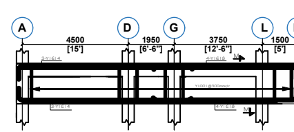
FLOOR BEAM ON G.L. 13 & 13a (2 NO)
