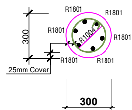
COL. BASE TYPE 'B2' ( 10 No. THUS )
