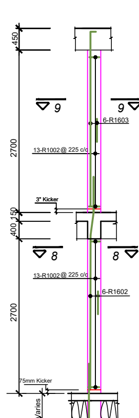
COLUMN TYPE 'C2' ( 54 No. THUS )
