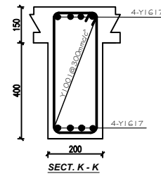
FLOOR BEAM ON G.L. 23, 25, 26 & 27 (4 NO)
