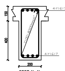
FLOOR BEAM ON G.L. 14, 15, 16 & 17 (4 NO)
