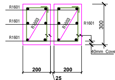
COL. BASE TYPE 'B3' ( 7 No. THUS )
