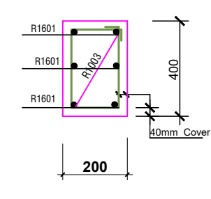
SECTION 16-16/17-17
