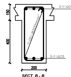
FLOOR BEAM ON G.L. D & G (2 NO)
