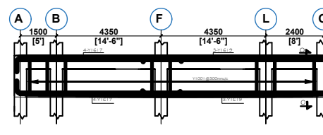
FLOOR BEAM ON G.L. 18 (1 NO)
