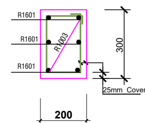
SECTION 6-6/7-7
