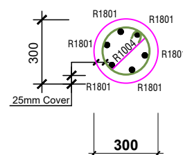
SECTION 8-8/9-9
