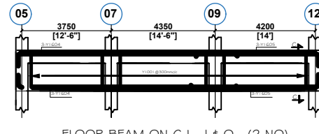
FLOOR BEAM ON G.L. J & O (2 NO)
