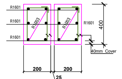
COL. BASE TYPE 'B5' ( 5 No. THUS )
