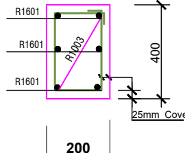
SECTION 12-12/13-13
