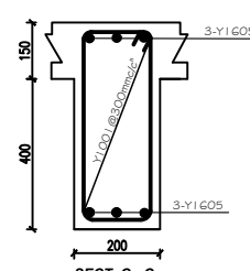
FLOOR BEAM ON G.L. 13 & 13a (2 NO)
