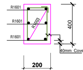
COL. BASE TYPE 'B4' ( 34 No. THUS )
