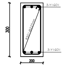
TYP. ROOF BEAM DETAIL
