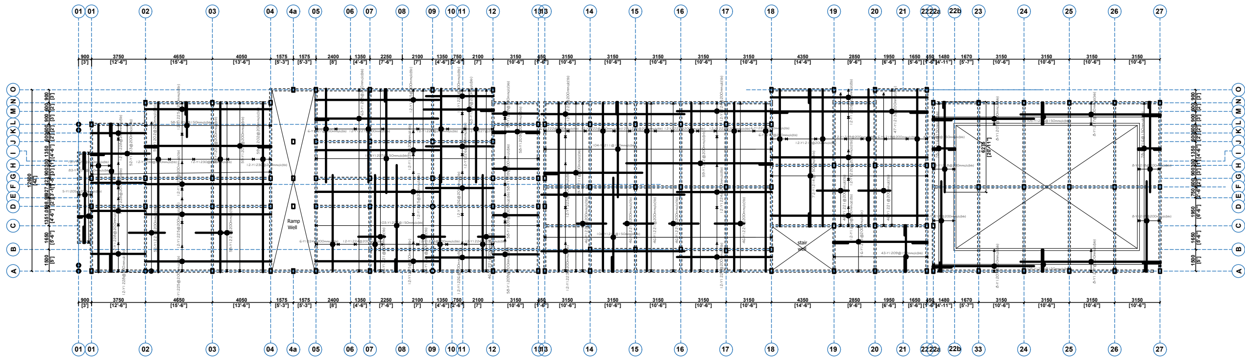
FIRST FLOOR SLAB DETAILS
