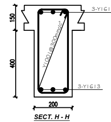
FLOOR BEAM ON G.L. A & H (2 NO)
