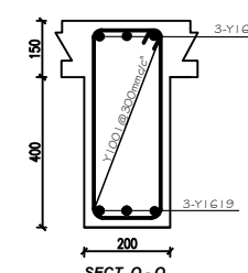
FLOOR BEAM ON G.L. 19 & 20 (2 NO)
