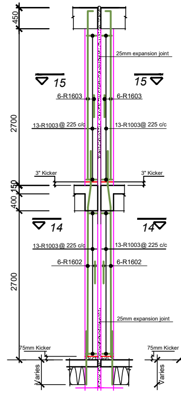
COLUMN TYPE 'C5' ( 5 No. THUS )
