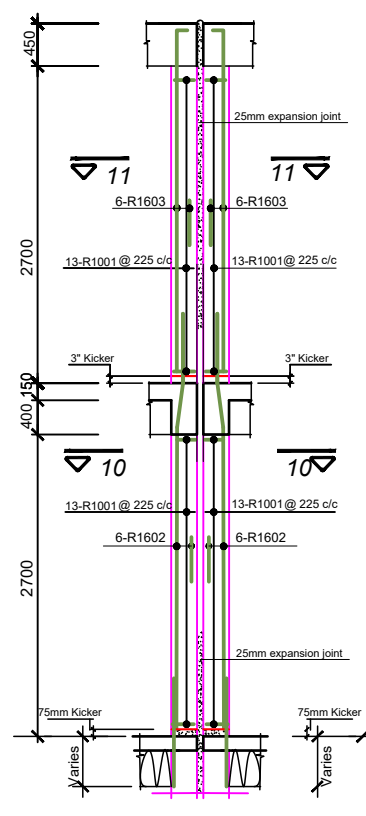
COLUMN TYPE 'C3' ( 5 No. THUS )
