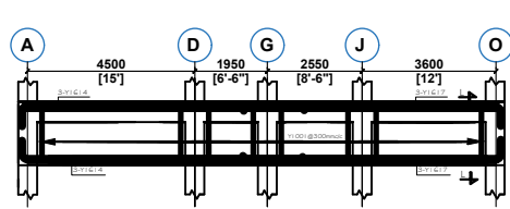
FLOOR BEAM ON G.L. 05, 07, 09, & 12 (4 NO)
