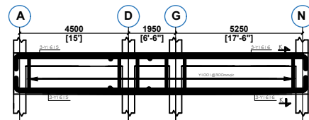
FLOOR BEAM ON G.L. 02, 03 & 04 (3 NO)
