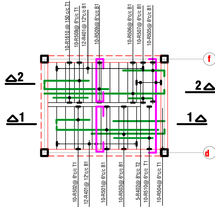
R.C STAIRCASE DETAILS FROM GROUND FLOOR TO FIRST FLOOR
