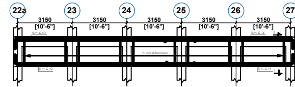
FLOOR BEAM ON G.L. A & N (2 NO)
