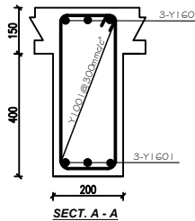
FLOOR BEAM ON G.L. N (1 NO)
