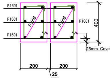
SECTION 14-14/15-15
