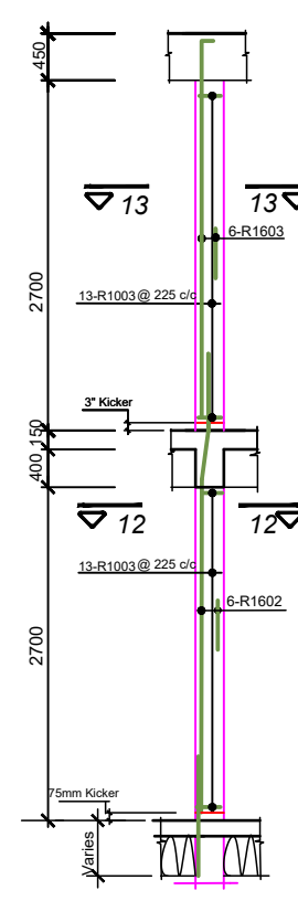
COLUMN TYPE 'C4' ( 54 No. THUS )
