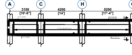
FLOOR BEAM ON G.L. 19 & 20 (2 NO)
