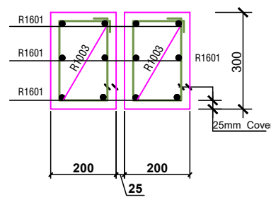
SECTION 10-10/11-11
