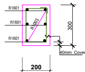
COL. BASE TYPE 'B1' ( 71 No. THUS )
